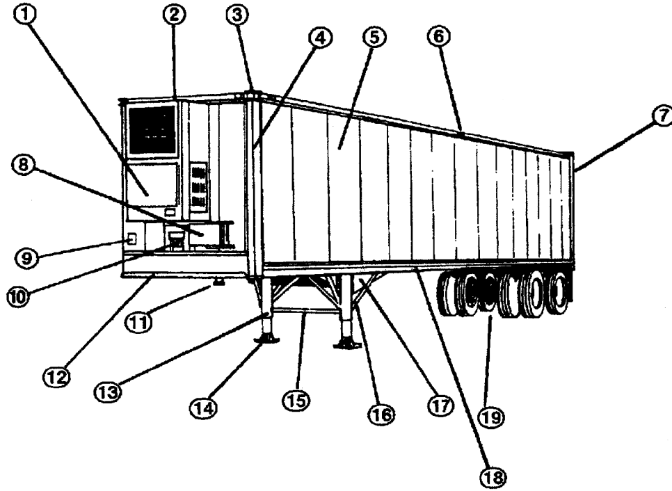
Figure C-1 Trailer Components—Front/Side
