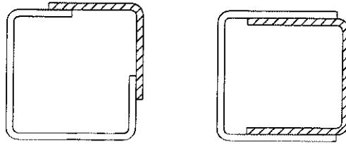
Figure B-14 Not Acceptable and Acceptable Rails
