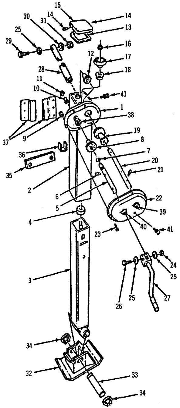
Figure B-5 Leg Assembly, Driver
