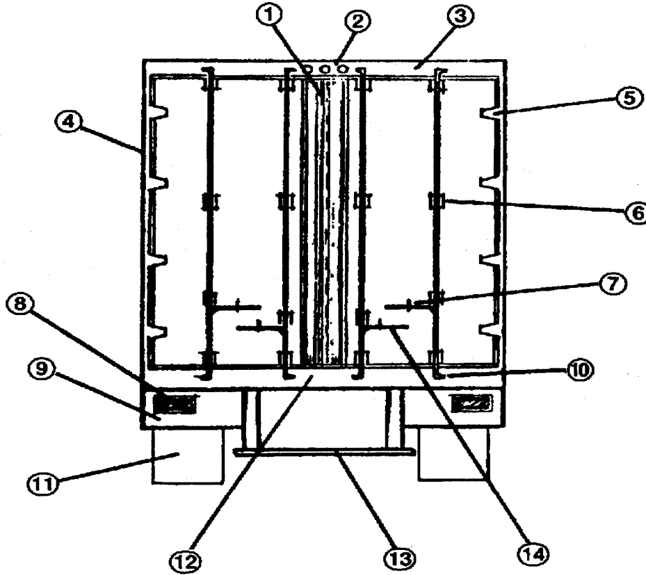
Figure C-2 Trailer Components—Rear
