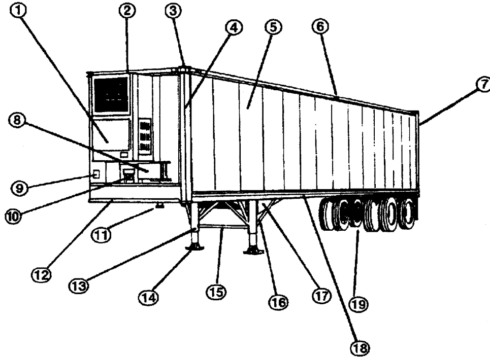
Figure C-1 Trailer Components—Front/Side
